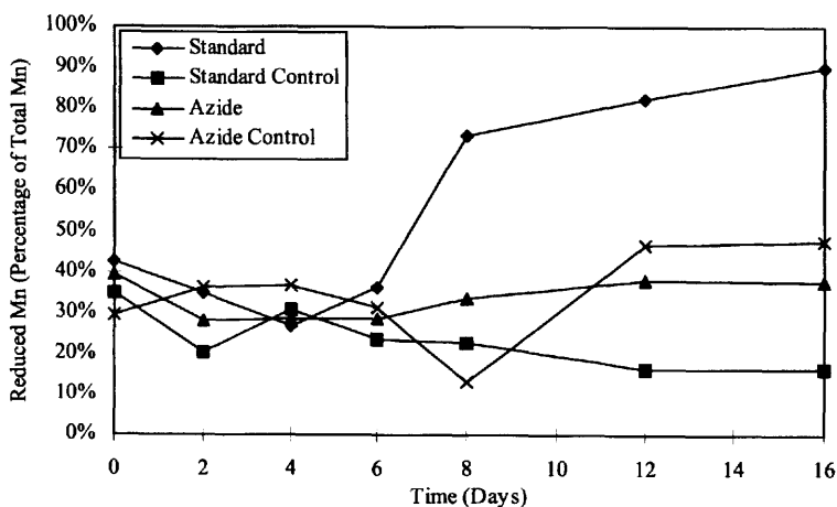
Figure 4. Percentage of reduced manganese ( Mn^{2+} ) in standard (anoxic; n=6 ), standard sterile control (anoxic; n=1 ), azide (anoxic; n=3 ) and azide sterile control (anoxic; n=1 ) microcosms. Statistical analysis of data presented in Table 1.
