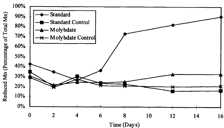
Figure 5. Percentage of reduced manganese ( Mn^{2+} ) in standard (anoxic; n=6 ), standard sterile control (anoxic; n=1 ), molybdate (anoxic; n=3 ) and molybdate sterile control (anoxic; n=1 ) microcosms. Statistical analysis of data presented in Table 1.
