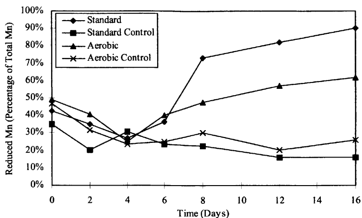
Figure 2. Percentage of reduced manganese ( \text{Mn}^{2+} ) in standard (anoxic; n=6 ), standard sterile control (anoxic; n=1 ), aerobic ( n=3 ) and aerobic sterile control ( n=1 ) microcosms. Statistical analysis of data presented in Table 1.
