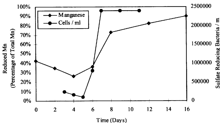
Figure 6. Percentage of reduced manganese ( \text{Mn}^{2+} ) ( n=6 ) and sulfate reducing bacteria (cells/ml) ( n=1 ) in standard anoxic microcosms.
