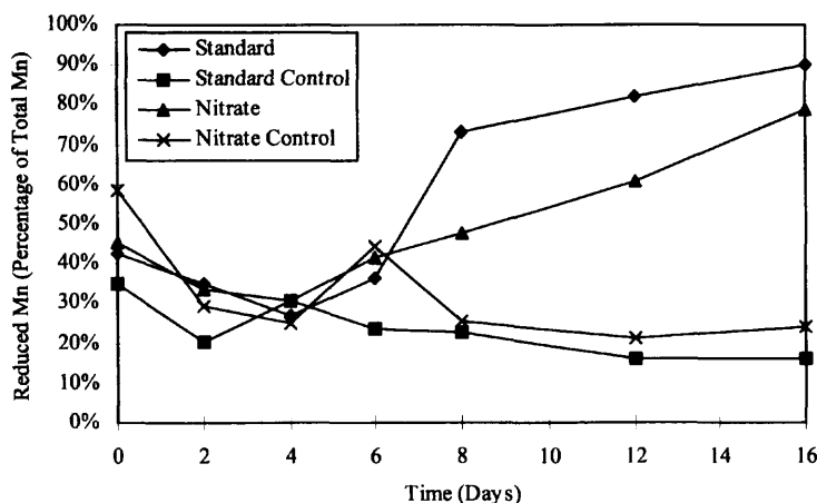
Figure 3. Percentage of reduced manganese ( Mn^{2+} ) in standard (anoxic; n=6 ), standard sterile control (anoxic; n=1 ), nitrate (anoxic; n=3 ) and nitrate sterile control (anoxic; n=1 ) microcosms. Statistical analysis of data presented in Table 1.
